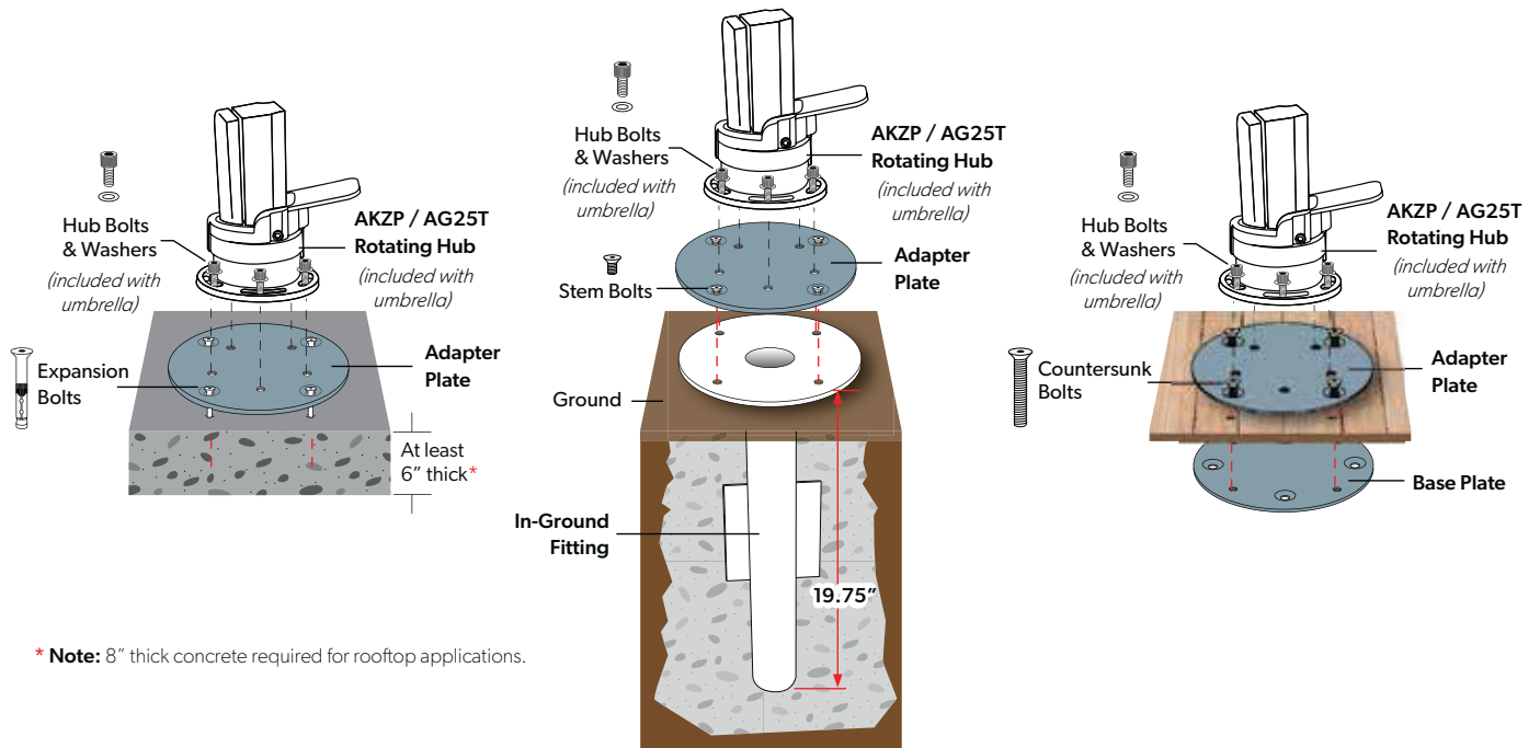
In-Ground Mount Includes: Adapter plate, in-ground fitting, and stem bolts
